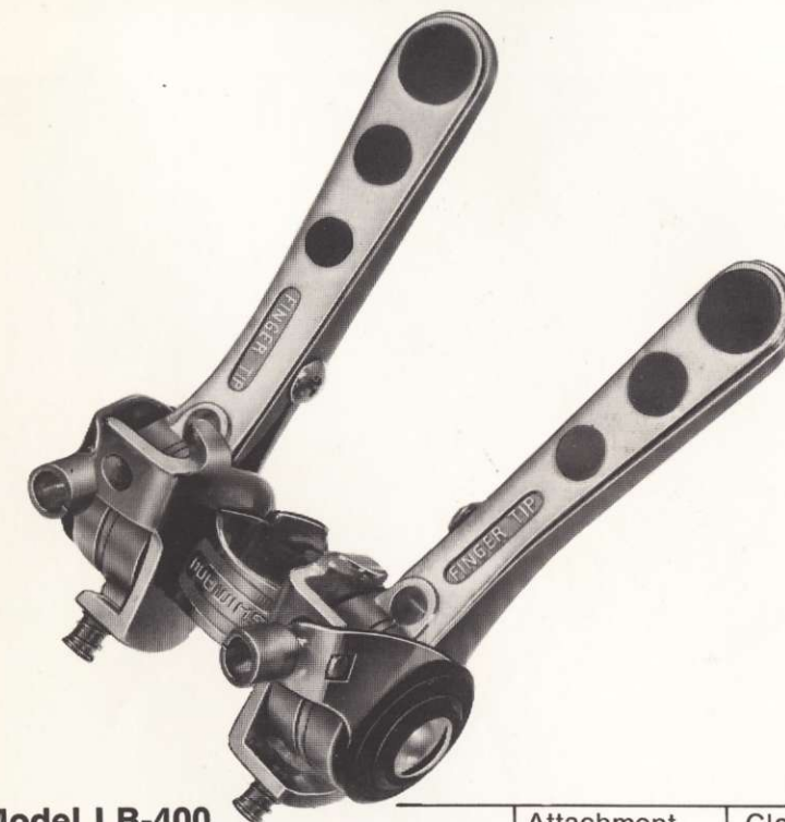
Model LB-400 FINGER-TIP SPECIFICATIONS Material: Light Alloy Type: With Spiral Spring (Balance Spring)
