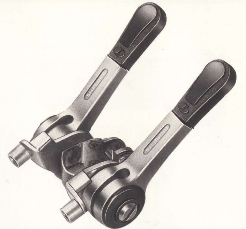
Model LB-300 SUPER SHIFTER SPECIFICATIONS Material: Light Alloy Type: One Way Clutch (With Special Cam)
