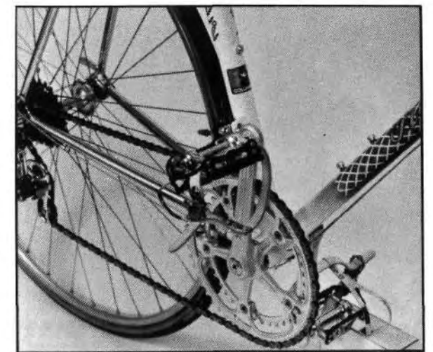
Campagnolo Super Record Group, Fully Engraved
